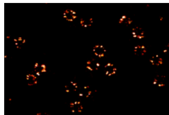
MINFLUX 2D
